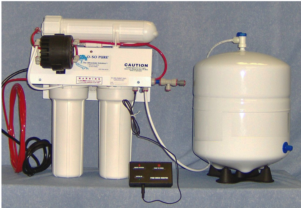
DWS-008 Ultimate Dominator operator water purification system
